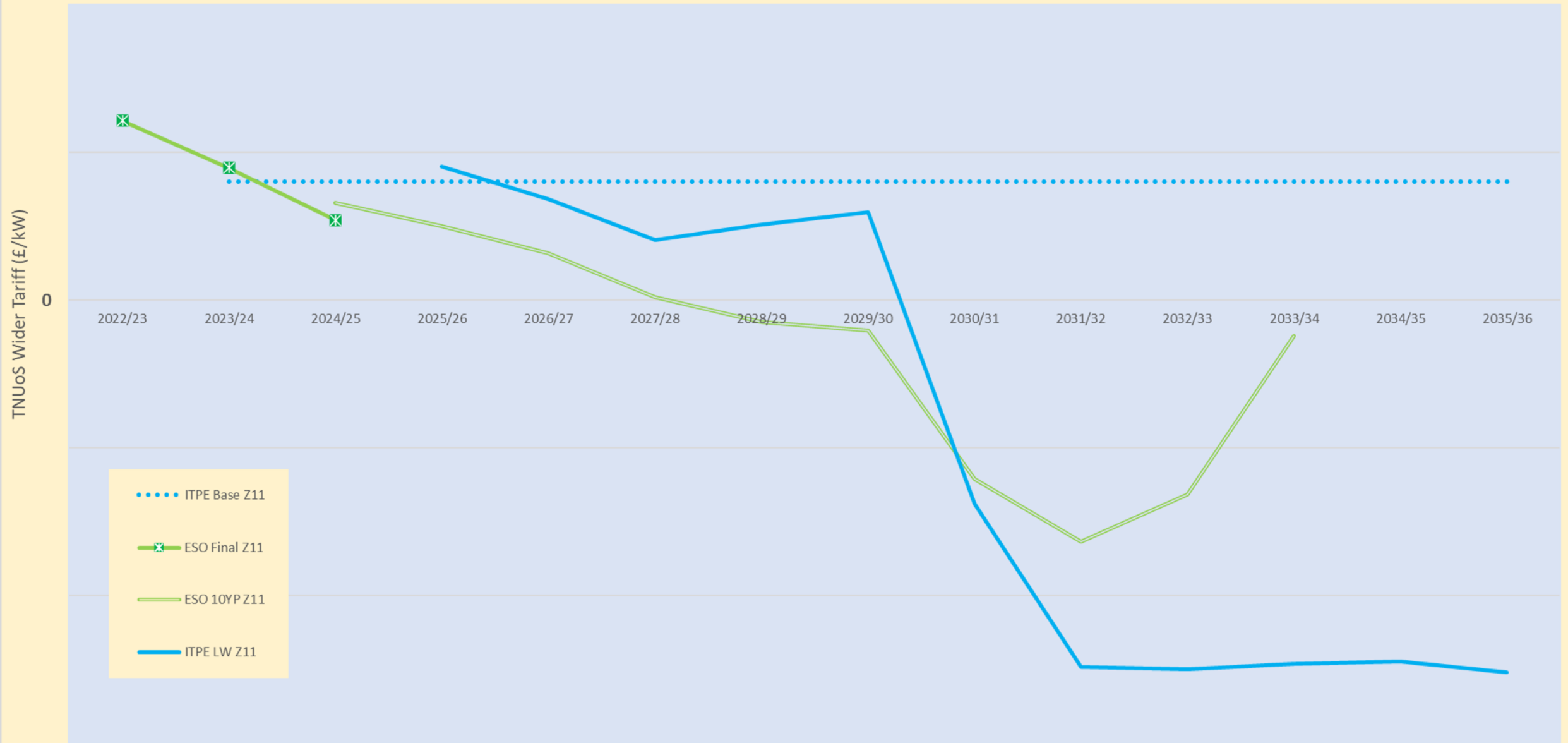
Estimated TNUoS Wider Tariffs Over Time - Zone 11, Money Of Year, BESS (Conventional Generation) with 9.8% ALF.
